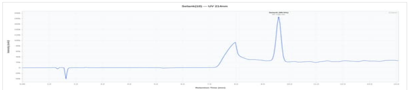
Selank 10 - PPA-CP-SK10-C6001: UV Chromatogram
