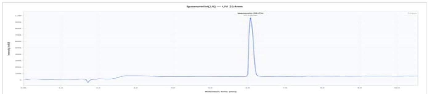
Ipamorelin 10 - PPA-CP-IP10-C6001: UV Chromatogram
